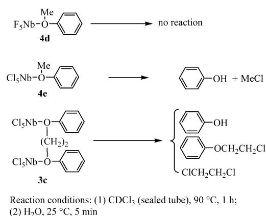
Scheme 3. Thermal stability of niobium complexes.
