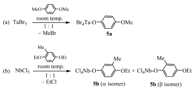
Scheme 4. Formation of aryloxy complexes from \text{MX}_5 and dialkoxarenes.
