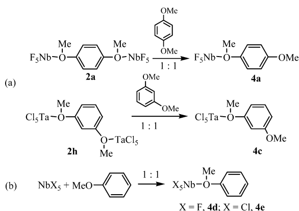
Scheme 1. Preparation of 1:1 adducts.
