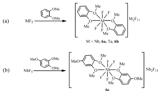
Scheme 5. Reactivity of \text{MF}_5 with ortho -methoxy-substituted benzenes.
