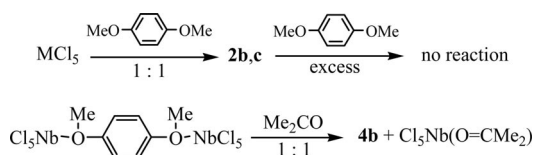
Scheme 2. Formation of dinuclear and mononuclear derivatives.
