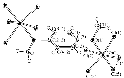
Figure 1. View of the molecular structure of 2b . Displacement ellipsoids are at the 50% probability level. Only one of the two independent molecules is represented. An inversion centre is located in the centre of the aromatic ring, generating the whole molecule (the underscore x_2 refers to symmetry-generated atoms by operation #1).
